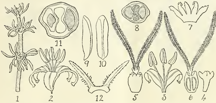
FIG. 1. Nenax acerosa , Gaertn. 1. Portion of male plant (natural size). 2. Male flower (side view) \times 5 . 3. Portion of the male corolla with the stamens attached \times 5 . 4. Calyx of male flower \times 20 . 5. Female flower \times 5 . 6. Longitudinal section of female flower \times 5 . 7. Corolla of female flower, laid out \times 10 . 8. Cross section through ovary \times 10 . 9 and 10. Ovules \times 5 . 11. Cross section through fruit \times 5 . 12. Pair of leaves, upper side, laid out \times 2 ( Salter 6376). Del. W. F. Barker.
